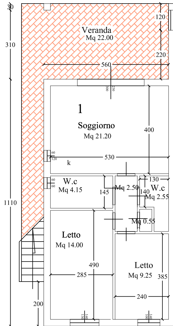
PIANO TERRA
