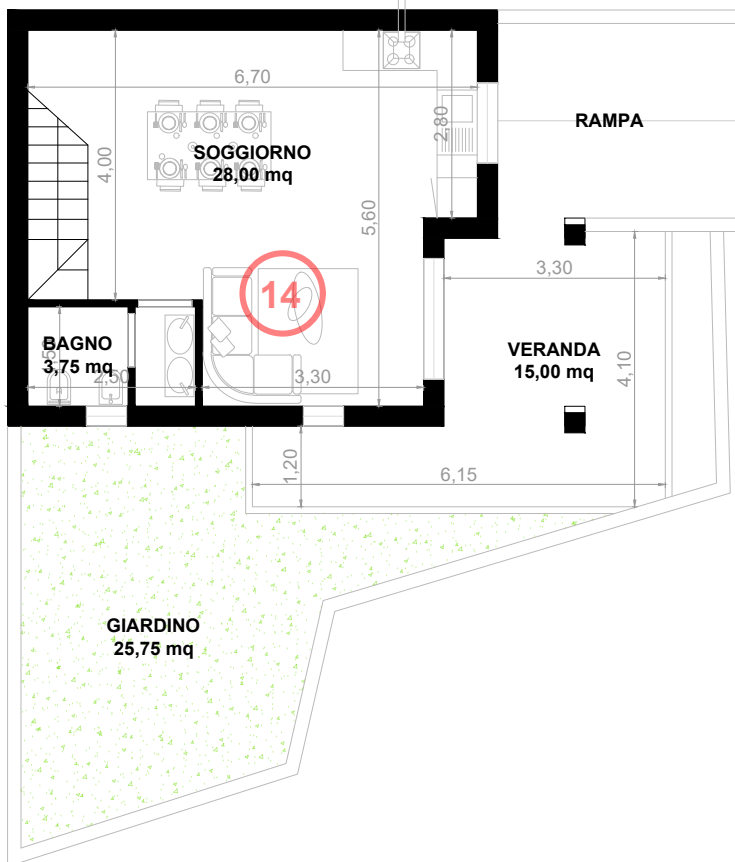
PIANO TERRA
